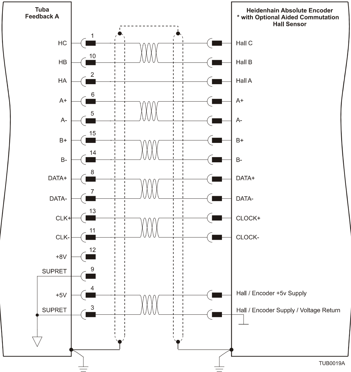
Figure 3-21: Main Feedback - Heidenhain Feedback Connection Diagram
