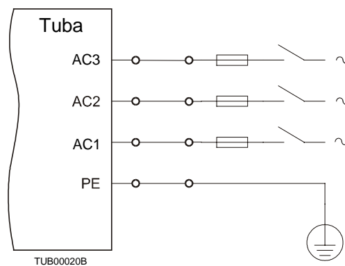
Figure 3-9: Main Power Supply Connection Diagram
