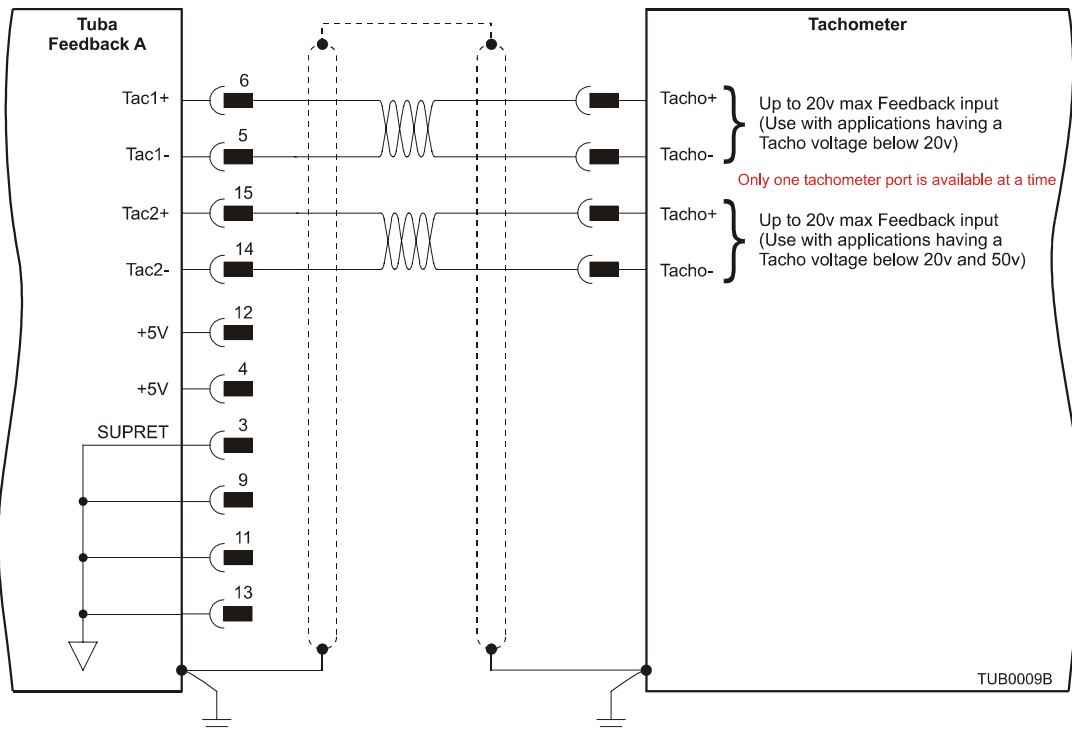
Figure 3-17: Main Feedback – Tachometer Feedback Connection Diagram
