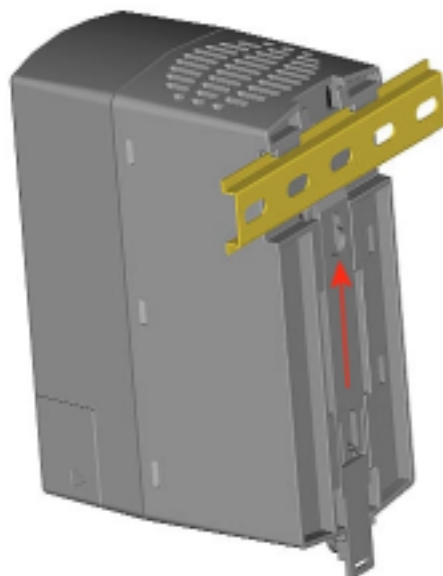
Figure 3-3: Attaching Top Part of Mounting Groove to DIN Rail
