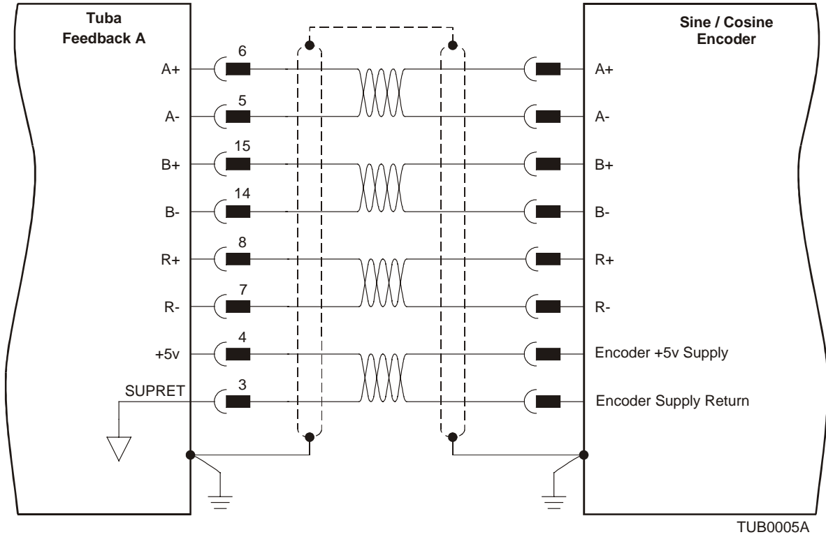
Figure 3-14: Main Feedback – Interpolated Analog Encoder Connection Diagram
