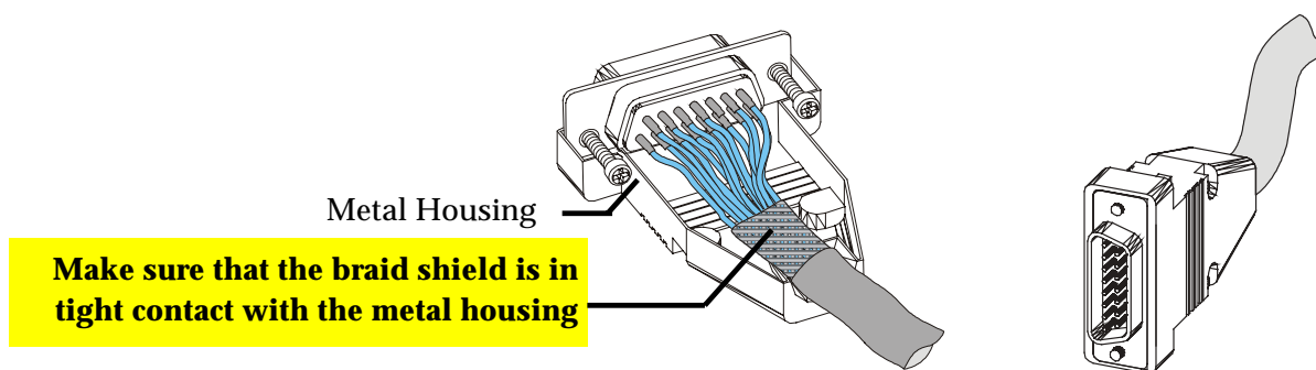
Figure 3-12: Feedback and Control Cable Assemblies
