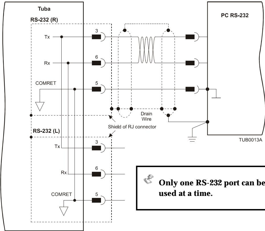
Figure 3-30: RS-232 Connection Diagram
